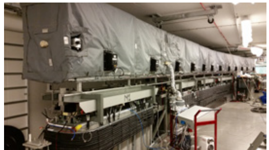
Bakeout tent, 23m long at MAX IV
